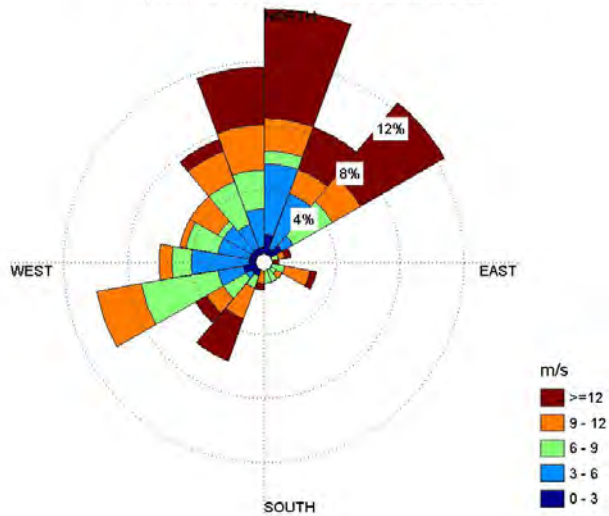
Medelvind, Vindstationen Hanö december 2010
